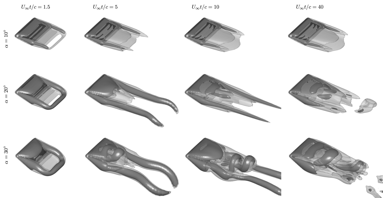
Fig. 1 Top-port snapshots of the wake vortices behind rectangular plates of AR = 2 at \alpha = 10, 20 , and 30 deg and the isosurfaces of \|\omega\|_2 = 2 and Q = 1 .
